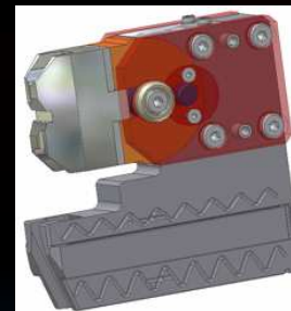
Pendulum clamping system to clamp elliptical parts
