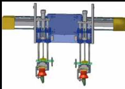
Workpiece exchange system with twist grippers
